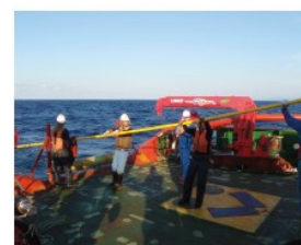
Lowering streamer cable into the sea
